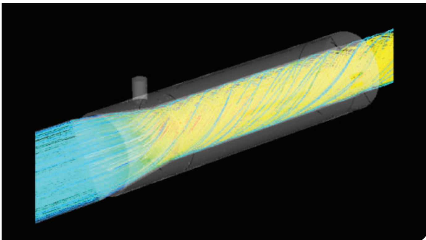
Above: The fully developed cyclone in the body of the inline device. The liquid rejection and gas recycle were removed for clarity.
